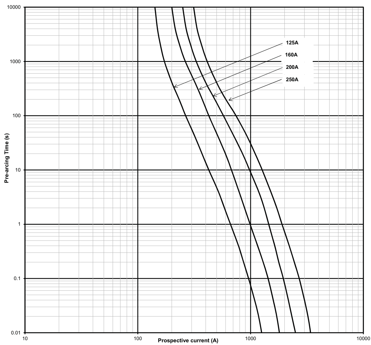
Time current curve - 1500 V d.c.- 2XL - Bladed and bolted
