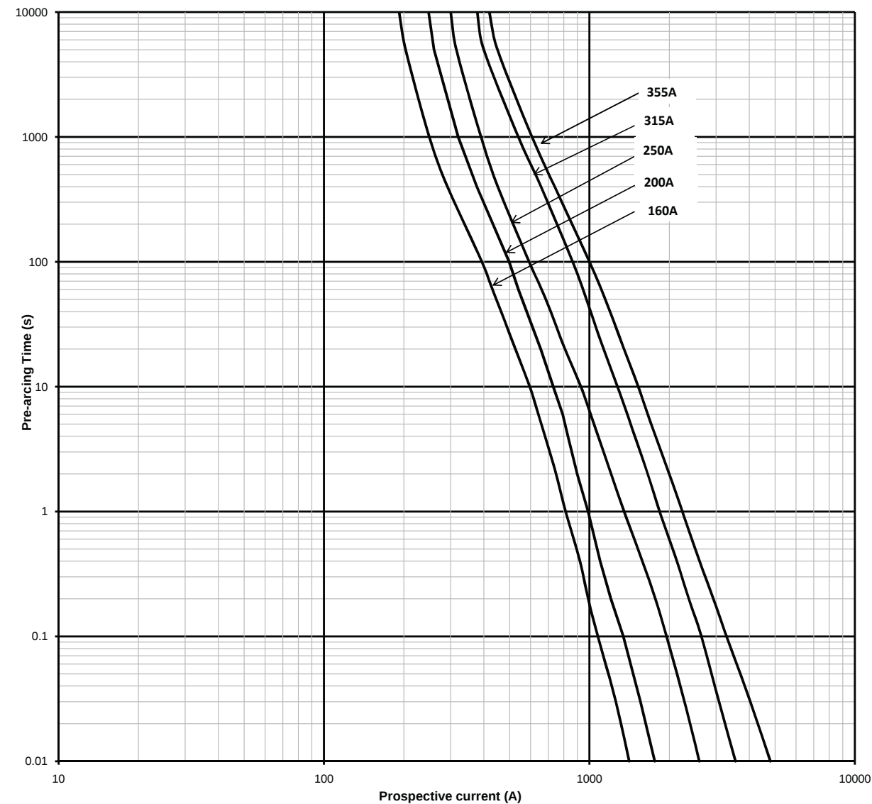
Time current curve - 1000 V d.c. - 2XL - Bladed and bolted
